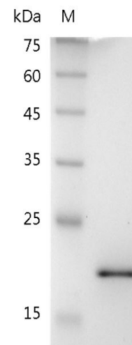
SDS-PAGE analysis of recombinant mouse TRAIL
